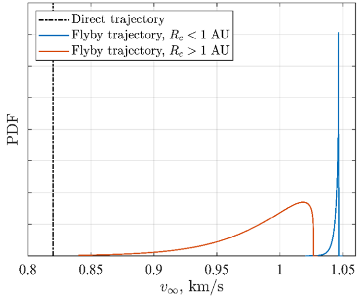
Figure a PDF of the escape velocities obtained from the Monte Carlo Simulation.
