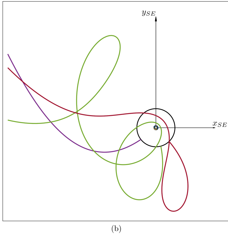
Figure 5.6: Examples of possible escape trajectories towards R_c > 1 AU (a) or towards R_c < 1 AU (b), identified respectively by \times and \bullet in Figure 5.5d.
