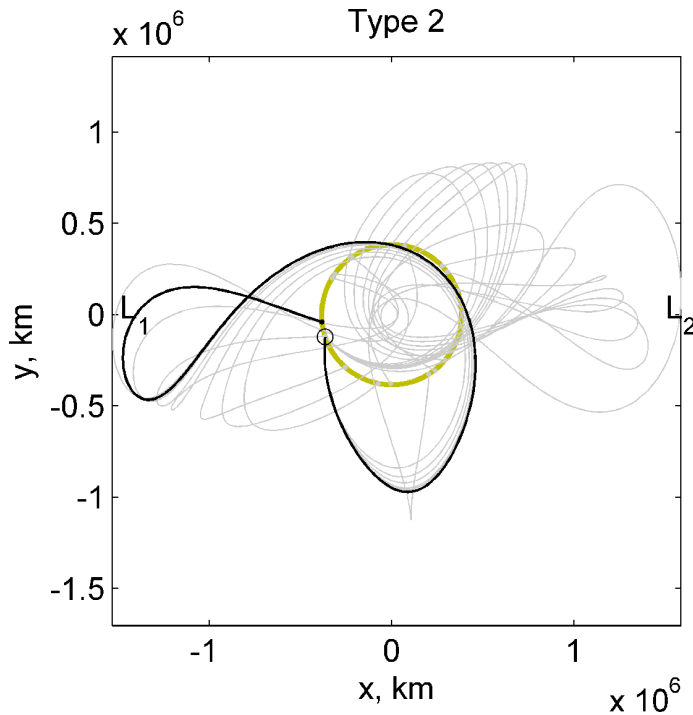
Figure 3.7: Example of a family of Moon-to-Moon transfers with two Sun-perturbed loops [44] .
