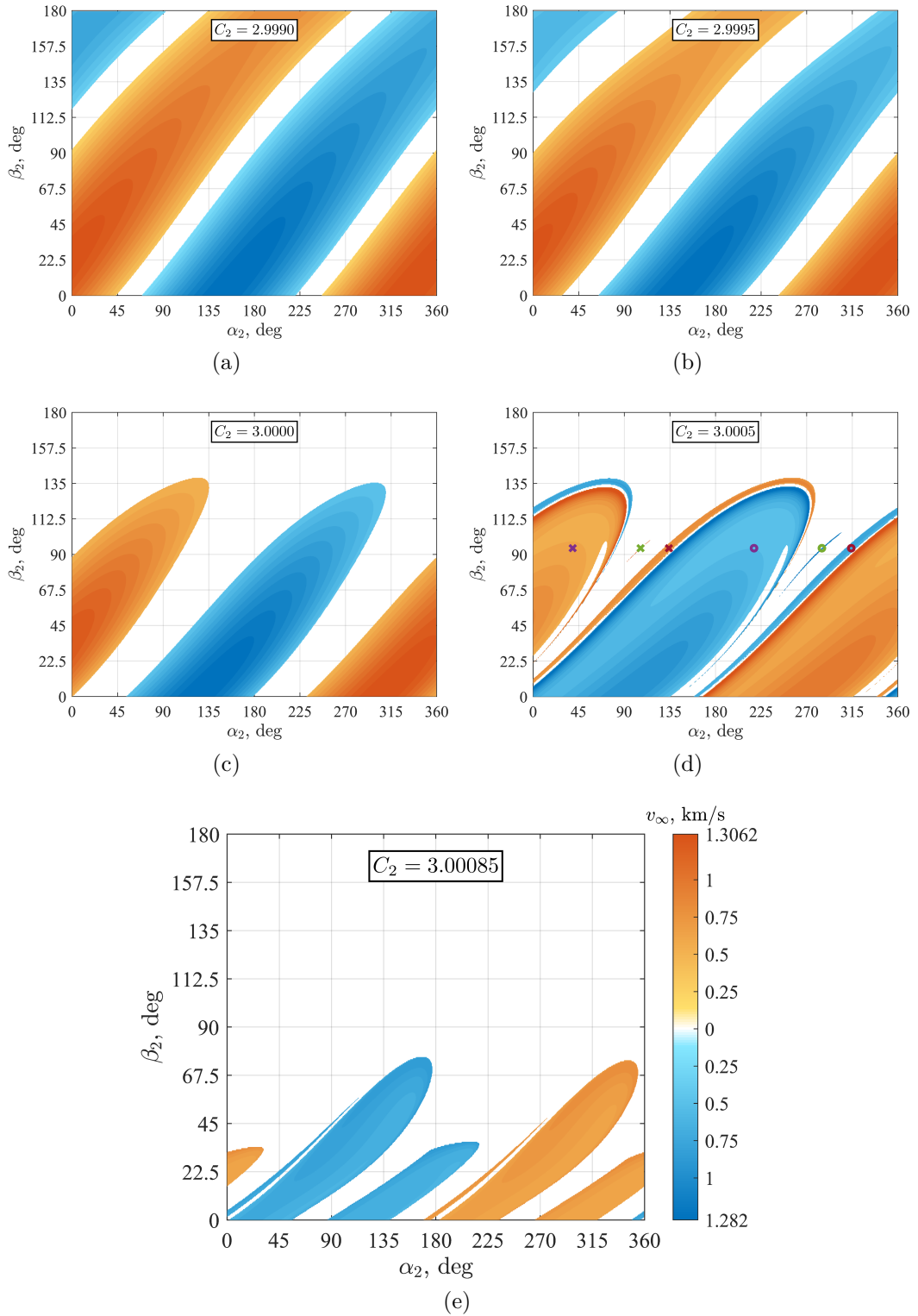
Figure 5.5: SOI SE Poincaré sections representing the escape velocity for a variety of Jacobi Constant levels. Trajectories departing towards R_c > 1 AU are in orange and trajectories departing towards R_c < 1 AU are in blue.
