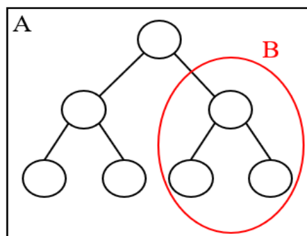
Figure 18: A binary tree and its subtree
