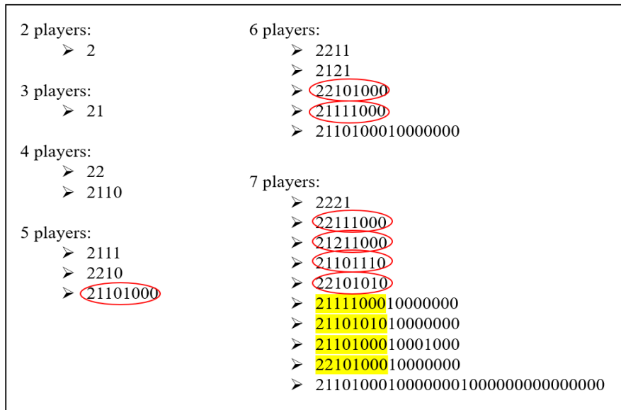
Figure 27: Labels for tournaments with up to seven players
