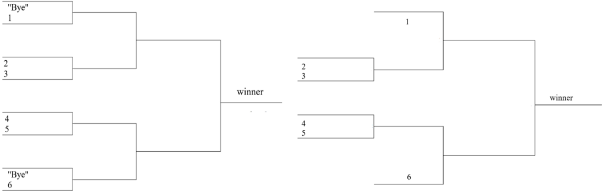
Figure 10: Six-player tournament structure with two “byes”
