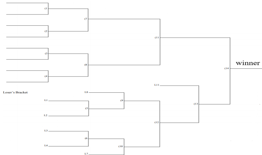
Figure 5: Double elimination bracket with eight participants. Retrieved from https://www.printyourbrackets.com/
