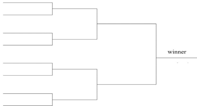
Figure 4: Single elimination bracket with eight participants
