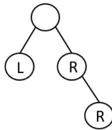
Figure 13: A binary tree with four nodes
