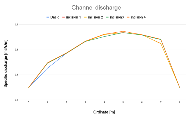
Figure 4.2: Mery Site - Discharge distribution due to incision gate openings at the cross-section in the intake channel
