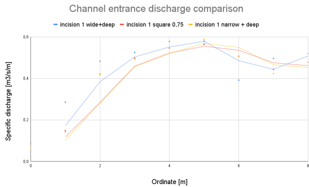
Figure 4.48: Mery Site - Channel entrance discharge incision 1 comparison
