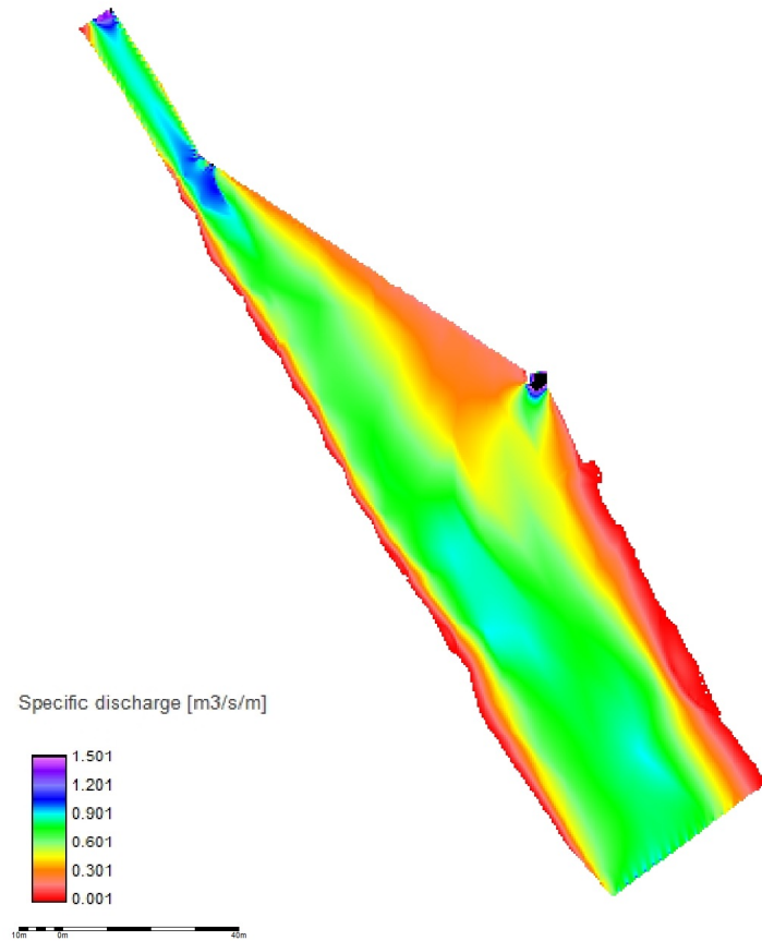
Figure 4.85: Mery Site - incision 1 specific discharge scenario 3
