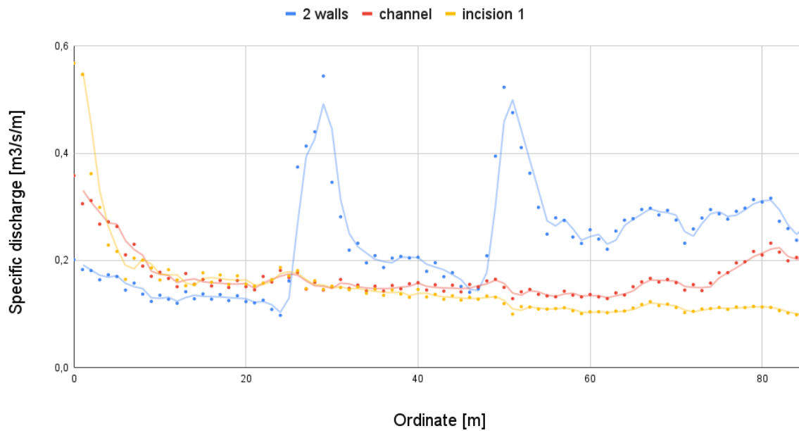
Figure 4.92: Mery Site - Specific discharge in front of the weir scenario 3 comparison
