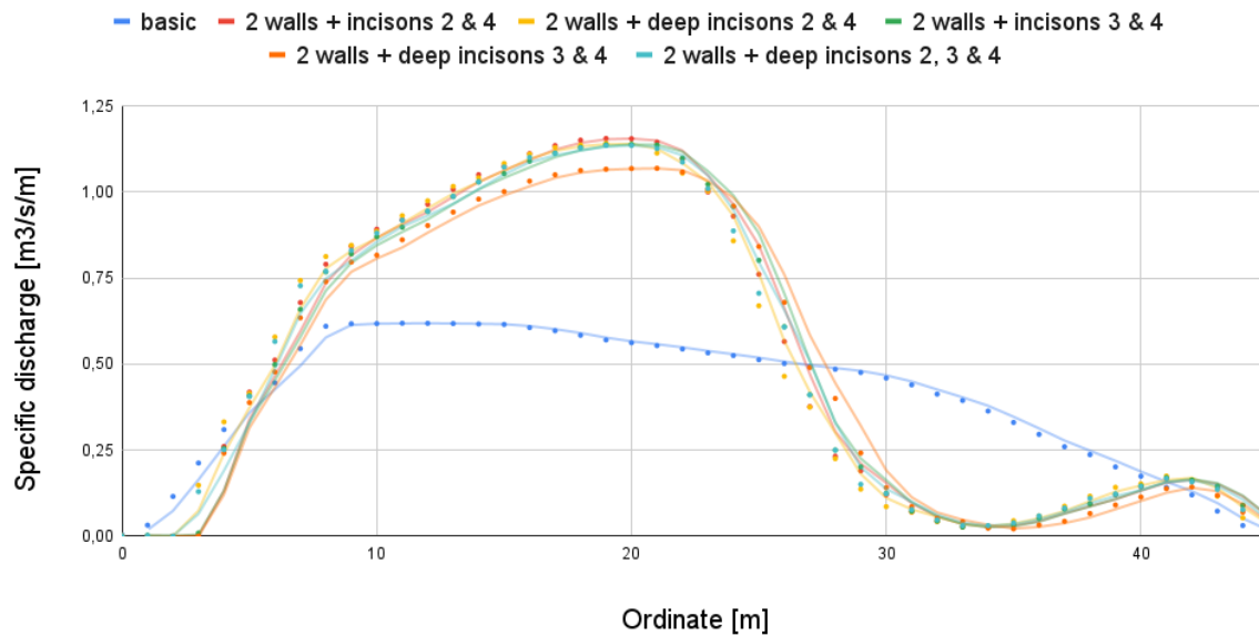
Figure 4.22: Mery Site - Main riverbed section 1 flow guide + incision comparison discharge distribution
