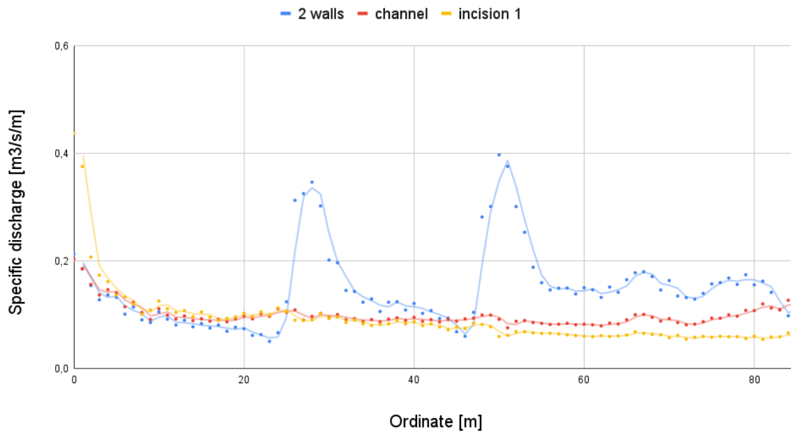
Figure 4.61: Mery Site - Specific discharge in front of the weir scenario 1 comparison
