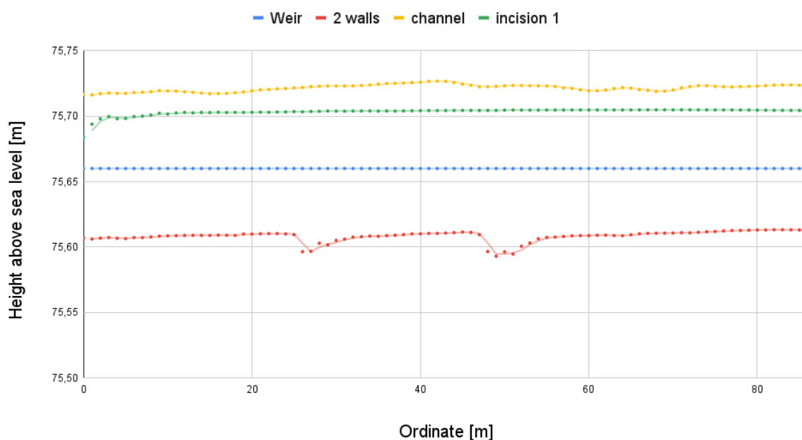
Figure 4.82: Mery Site - Weir section water level scenario 2 comparison
