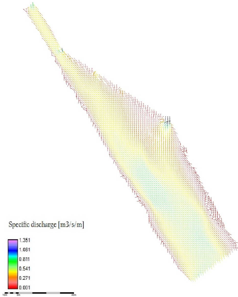
Figure C.7: Mery Site - Discharge vectors
