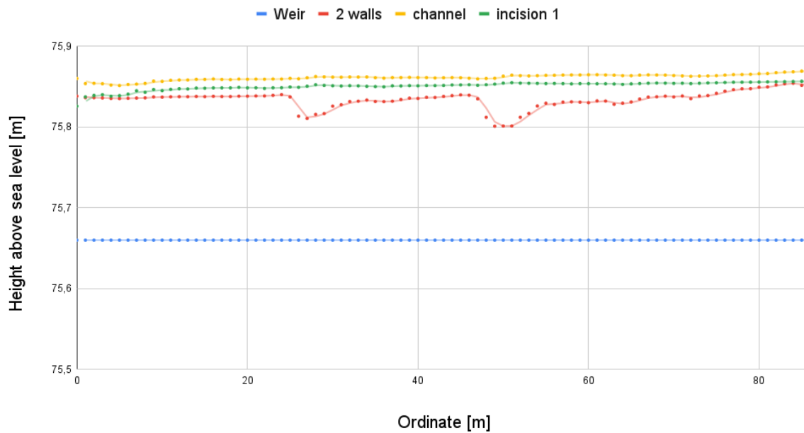
Figure 4.96: Mery Site - Weir section water level scenario 3 comparison
