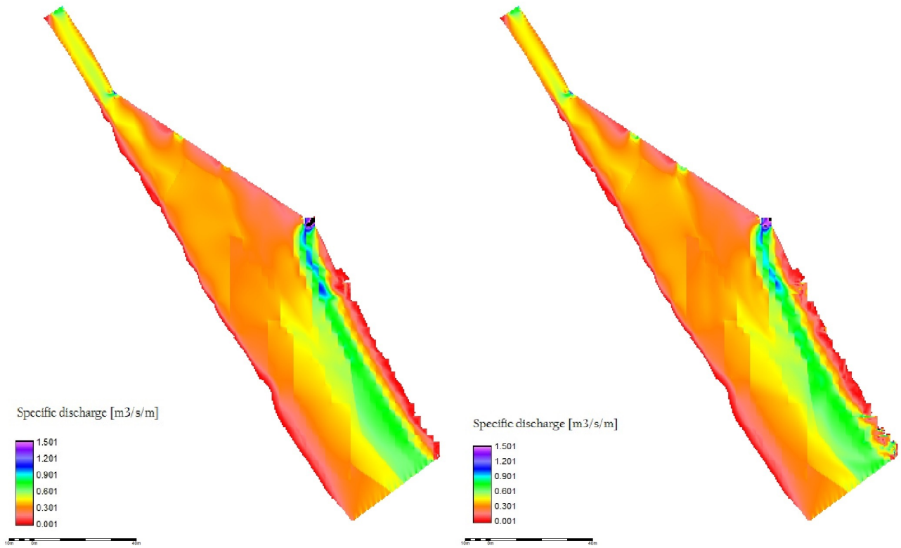
Figure 4.31: Mery Site - Channel displacement + incisions 2, 3 and 4 Figure 4.32: Mery Site - Channel displacement + deep incisions 2, 3 and 4
