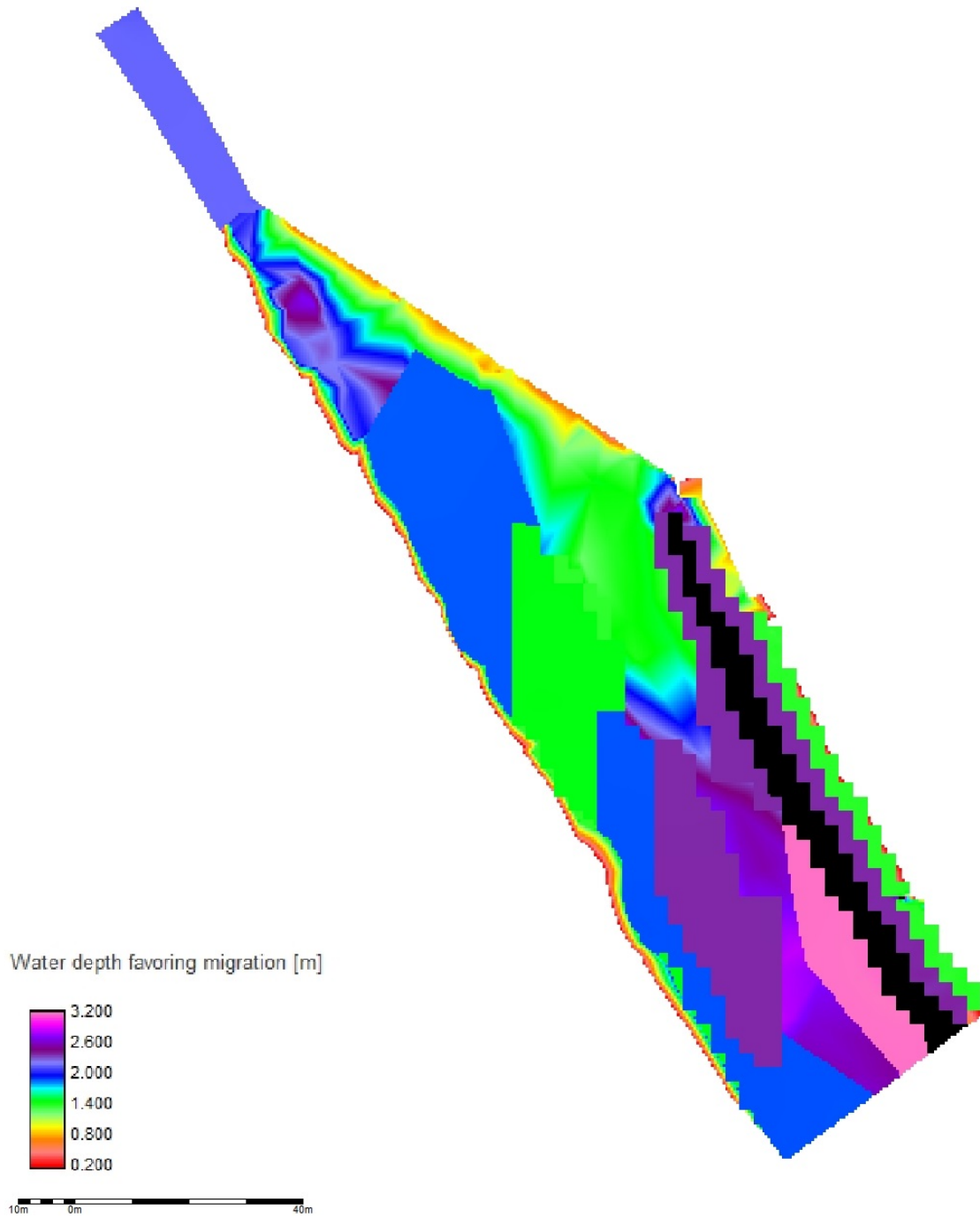
Figure D.15: Mery Site - channel displacement water depth favoring migration scenario 3
