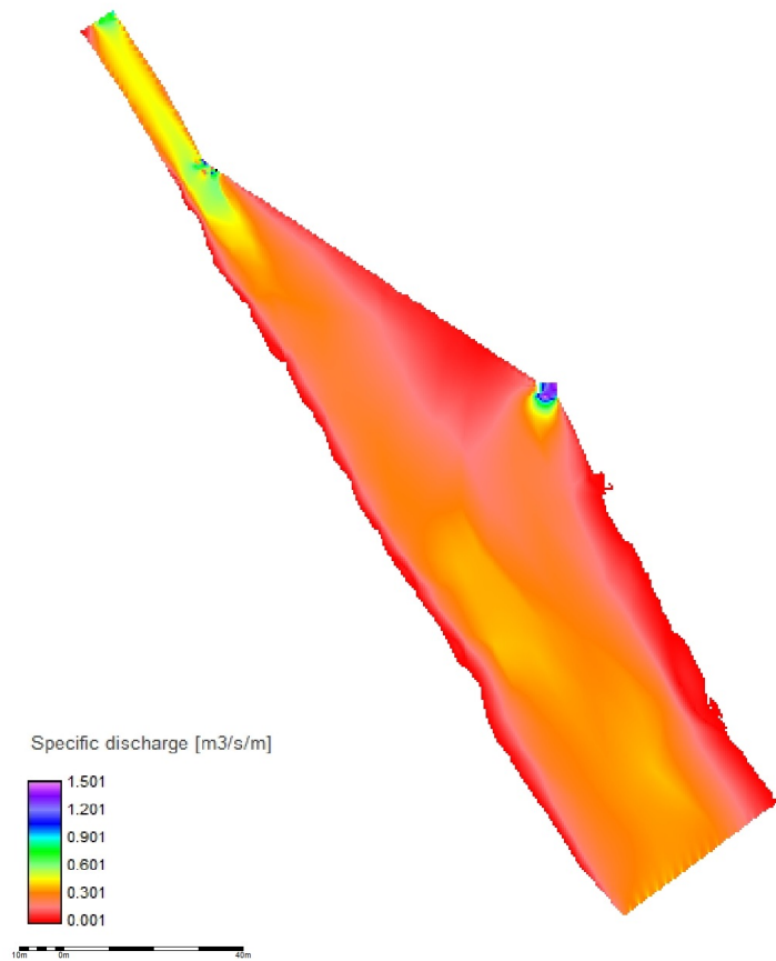
Figure 4.71: Mery Site - incision 1 specific discharge scenario 2
