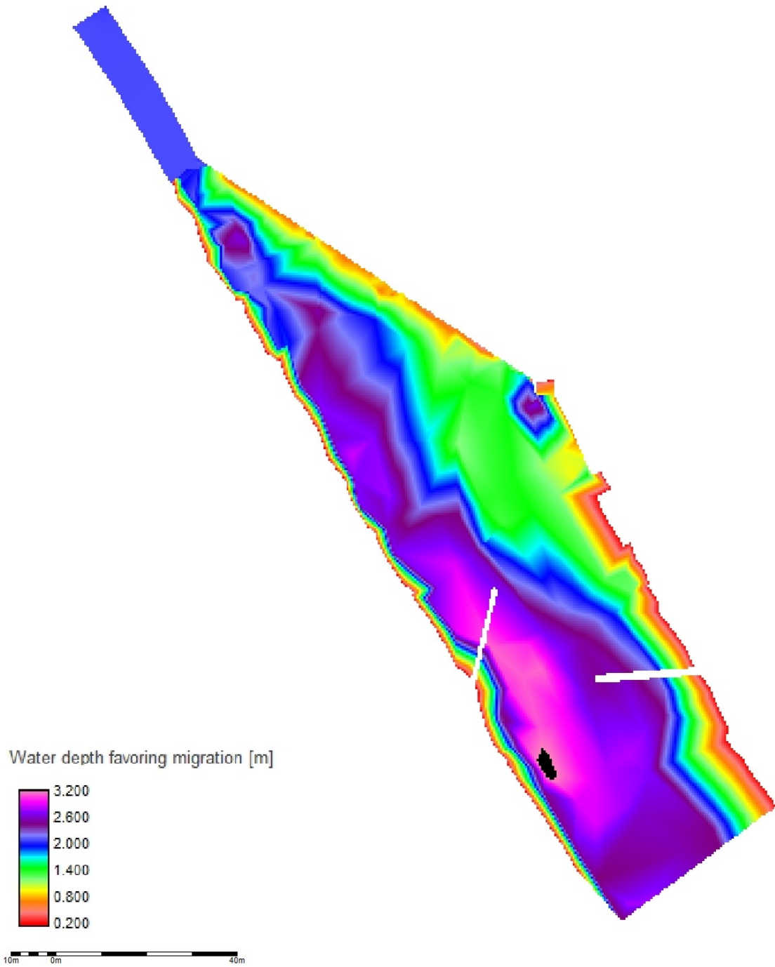
Figure D.14: Mery Site - 2 guiding walls water depth favoring migration scenario 3
