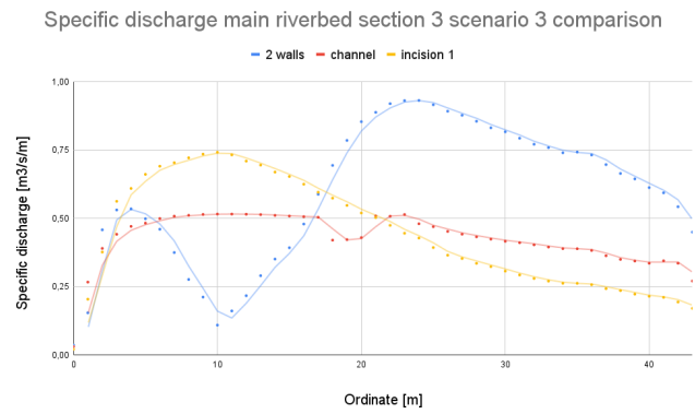
Figure 4.89: Mery Site - Main riverbed section 3 specific discharge scenario 3 comparison
