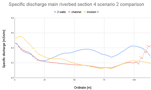
Figure 4.76: Mery Site - Main riverbed section 4 specific discharge scenario 2 comparison Figure 4.77: Mery Site - Main riverbed section 5 specific discharge scenario 2 comparison
