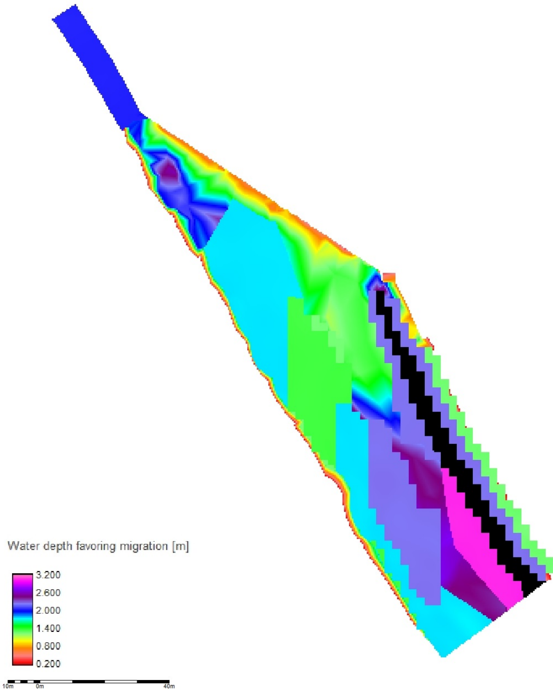
Figure D.12: Mery Site - channel displacement water depth favoring migration scenario 2
