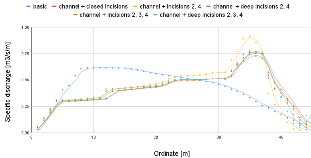
Main riverbed section 1 channel displacement + incisions combination comparison
