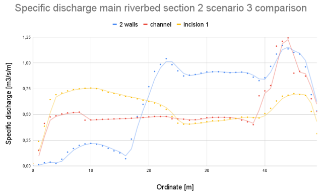
Figure 4.88: Mery Site - Main riverbed section 2 specific discharge scenario 3 comparison
