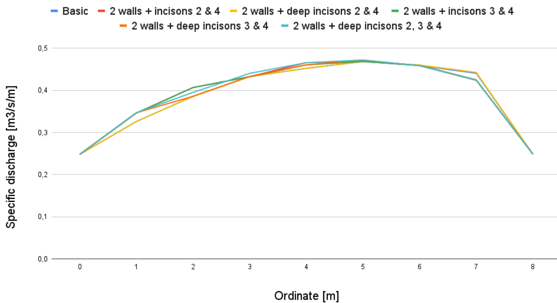
Figure 4.26: Mery Site - Channel section flow guide + incision comparison discharge distribution
