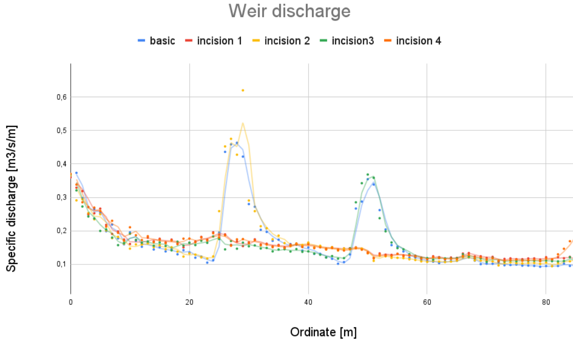
Figure 4.3: Mery Site - Discharge distribution due to incision gate openings at the cross-section in front of the weir
