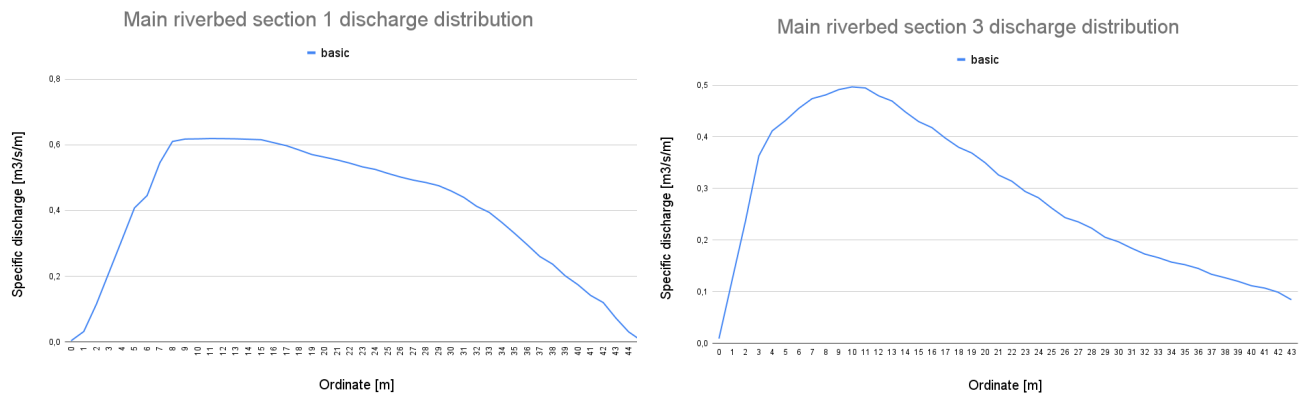
Figure 3.8: Mery Site - Discharge distribution at cross-section 1
