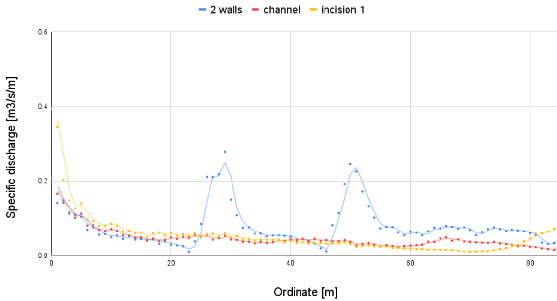
Figure 4.78: Mery Site - Specific discharge in front of the weir scenario 2 comparison
