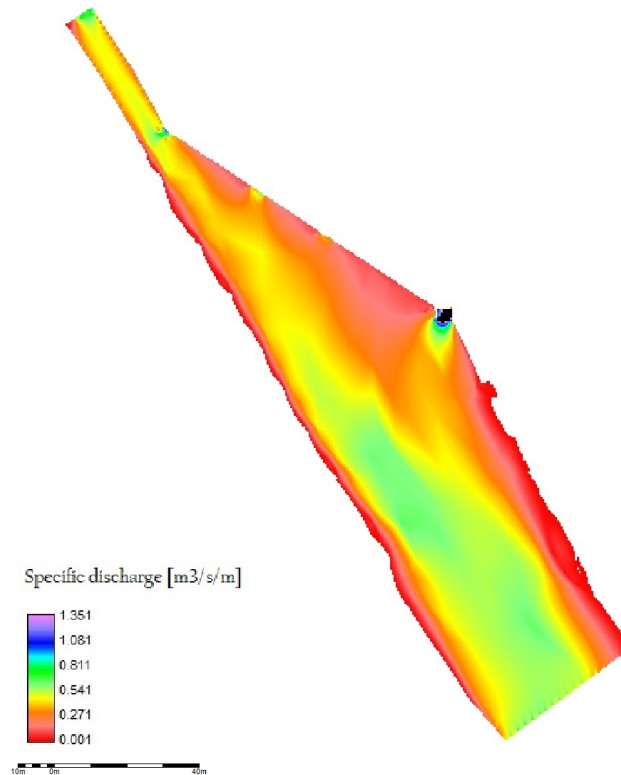
Figure 3.7: Mery Site - Discharge
