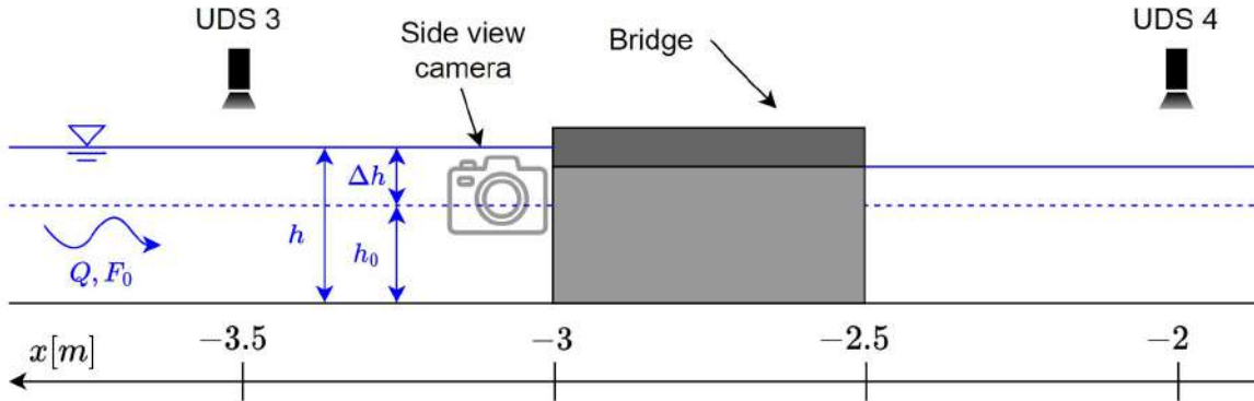
Figure 19: Side view of the experimental setup
