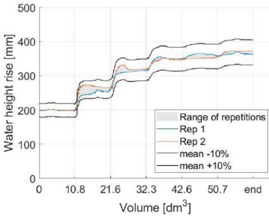
(a) h_0 = 200mm, Fr_0 = 0.60 , cubes, 1 pier.
