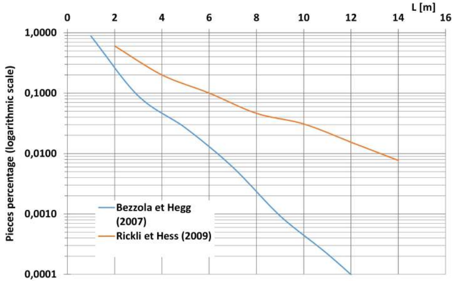
Figure 26: References size distribution of natural debris according to 2 studies.
