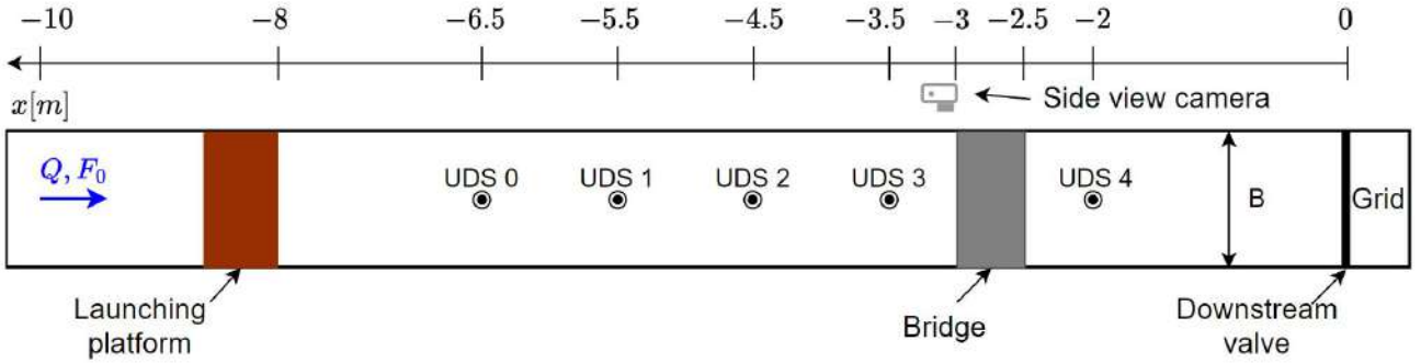
Figure 17: Plan view of the experimental setup and arrangement of UDS_s . Notations: B is the width of the flume, Q is the discharge and F_0 is the initial Froude number of the flow.
