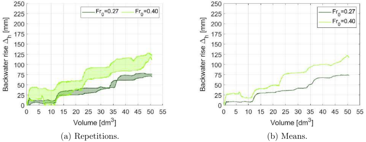
Figure 42: Backwater rise according to the added volume, cubes, h_0 = 240mm , 1 pier Comparison between the graph of the repetitions and the mean.
