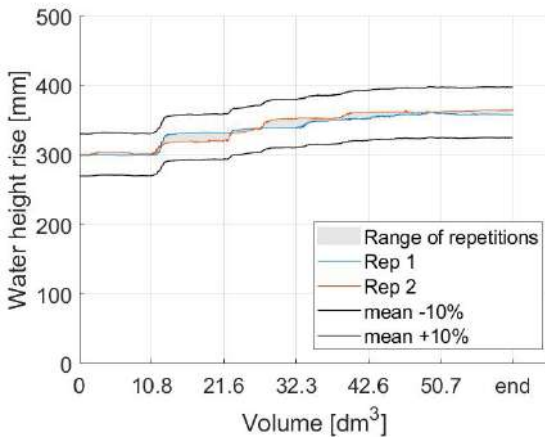
(c) h_0 = 310mm, Fr_0 = 0.27 , cubes, 2 piers.
