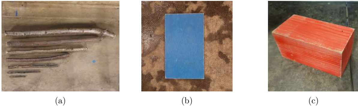
Figure 24: Debris types, (a) Natural wood, (b) 2D elements, (c) 3D elements.
