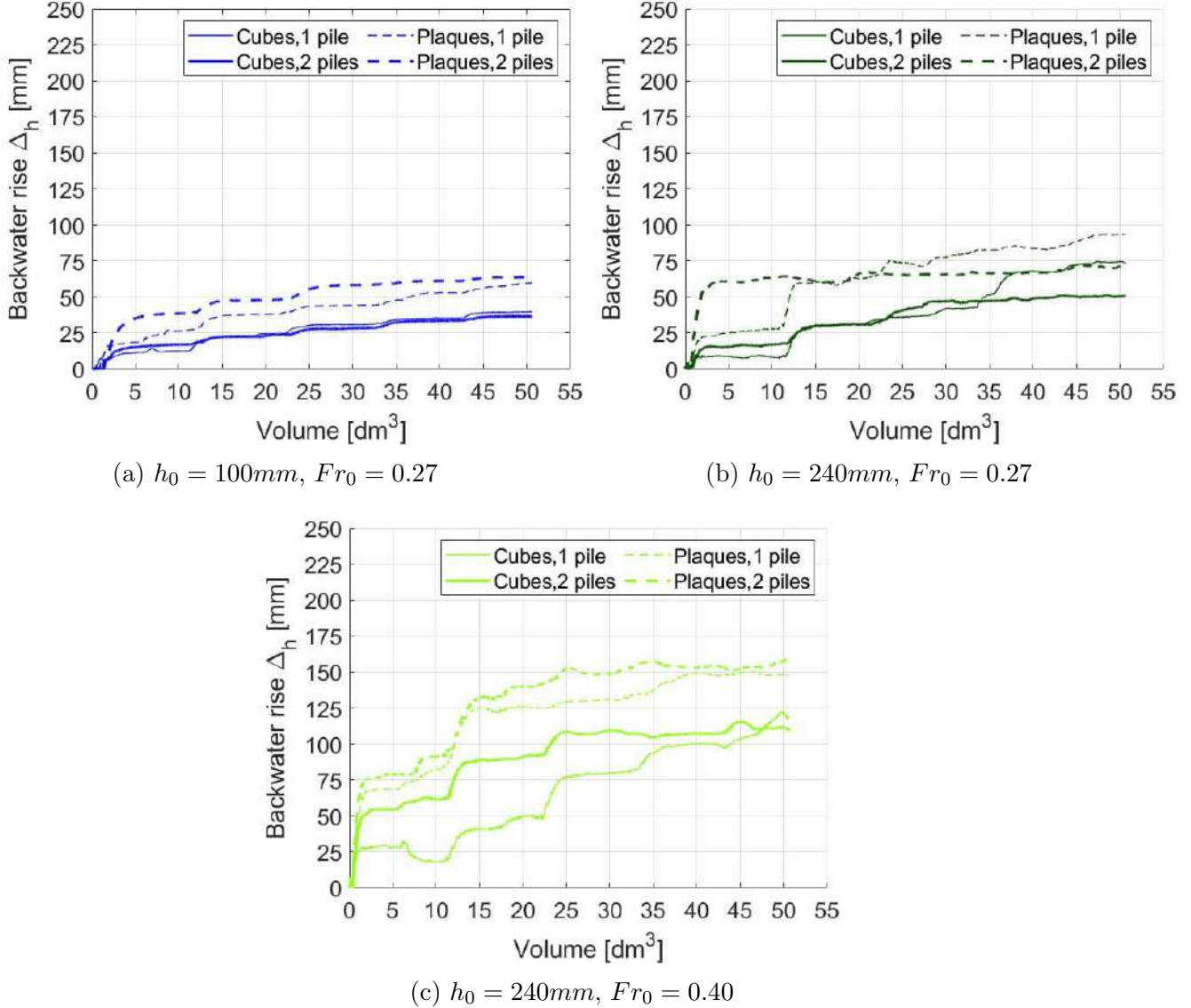
Figure 53: Backwater rise according to the added volume for both mixture (25 % cubes and 25 % plates) and both geometries (1 and 2 piers) for 3 representative configurations.
