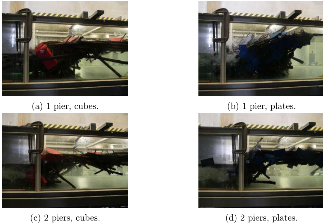
Figure 43: Comparison of the backwater rise for identical initial hydraulic conditions and variable bridge geometry and debris mixture.
