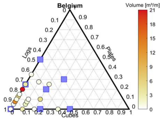
Figure 28: Tested mixture.
