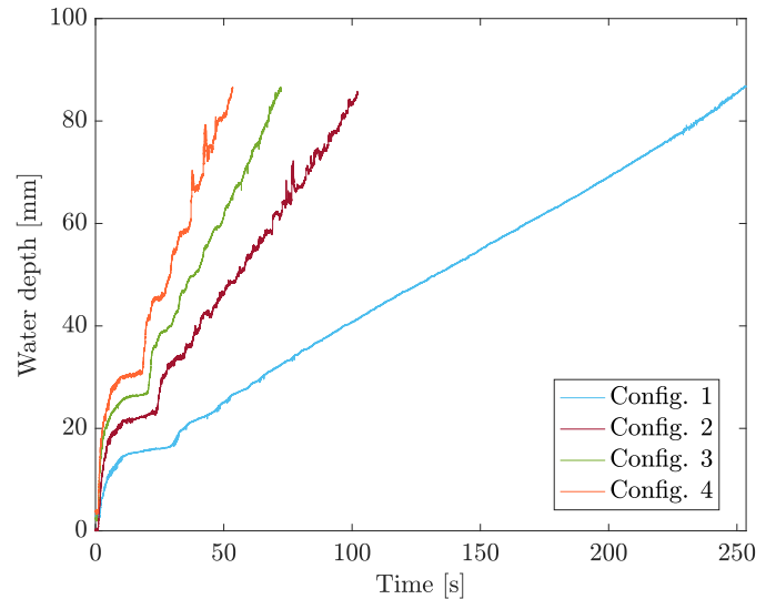
FIG. 47 Comparison between the four configurations for the first sensor with dimension variable
