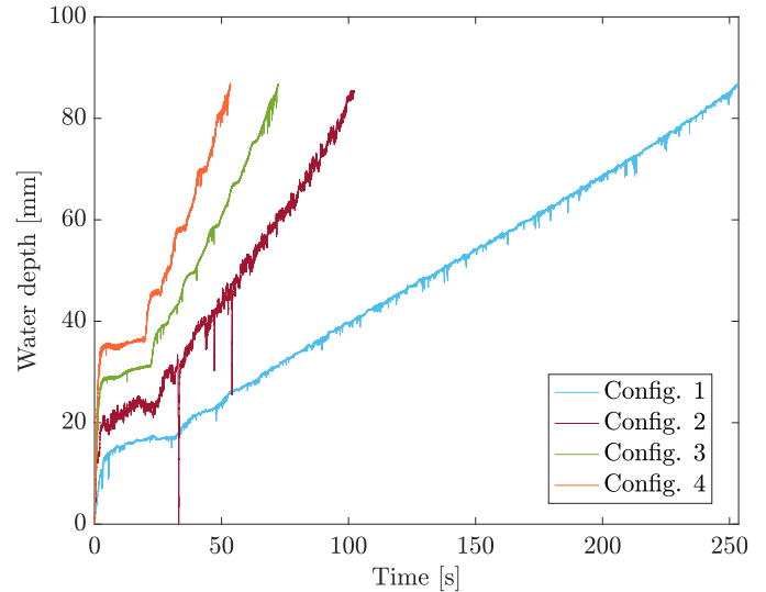
FIG. 51 Comparison between the four configurations for the sensor in the tank with dimension variables
