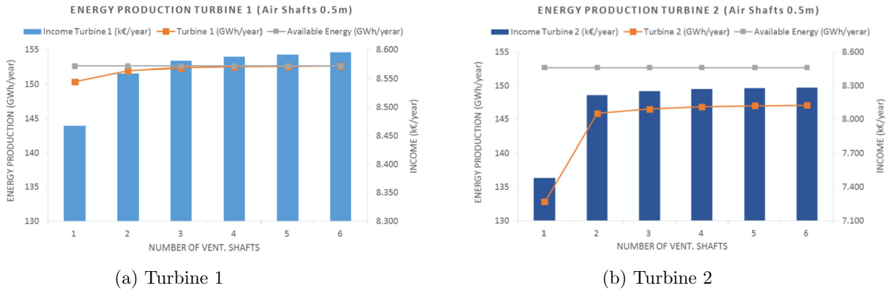
FIG. 1 Influence of the number of air shafts [Menendez et al., 2019]
