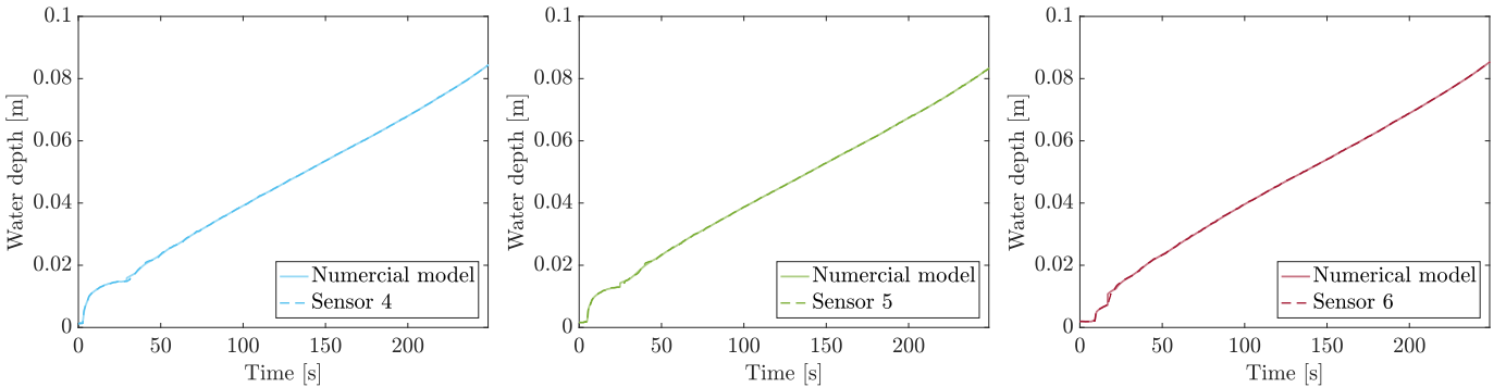
(a) Comparison between the numerical model and the sensor four
