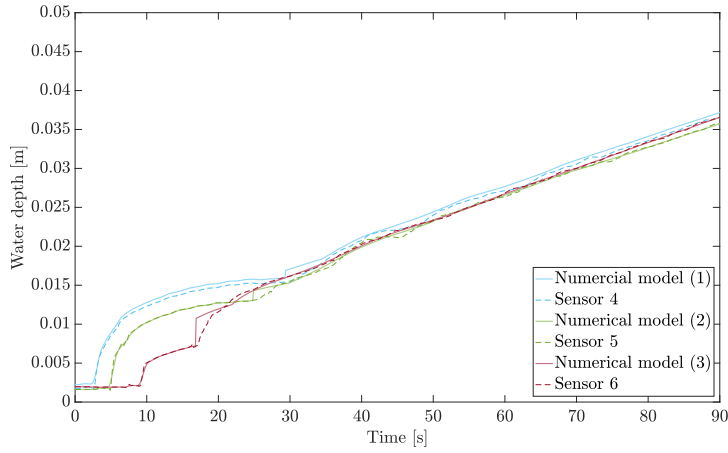
FIG. 34 Comparison between the numerical model and the laboratory measurement for the three last sensors (configuration one)
