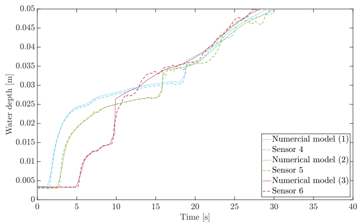
FIG. 36 Comparison between the numerical model and the laboratory measurement for the three last sensors (configuration four)
