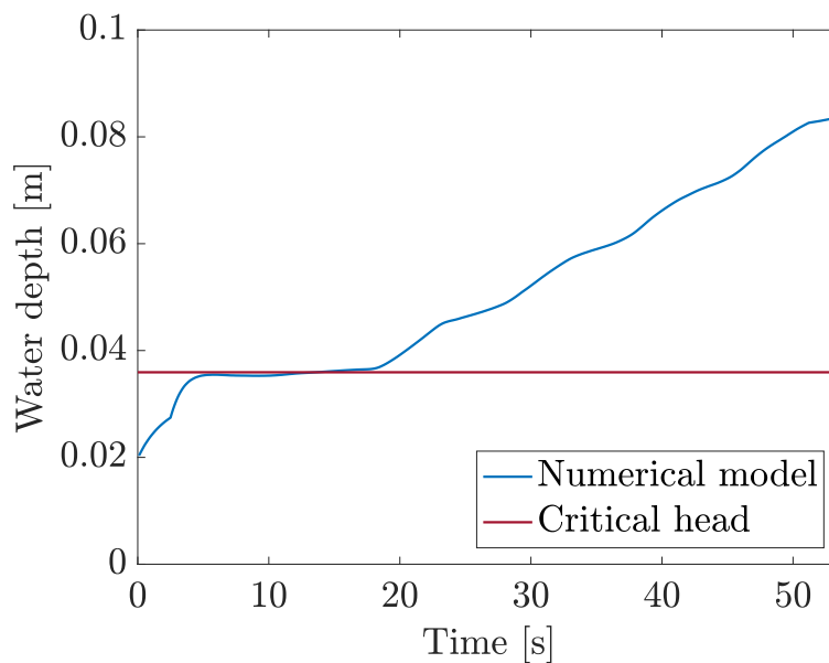
FIG. 33 Numerical curve in the tank compared with the critical head
