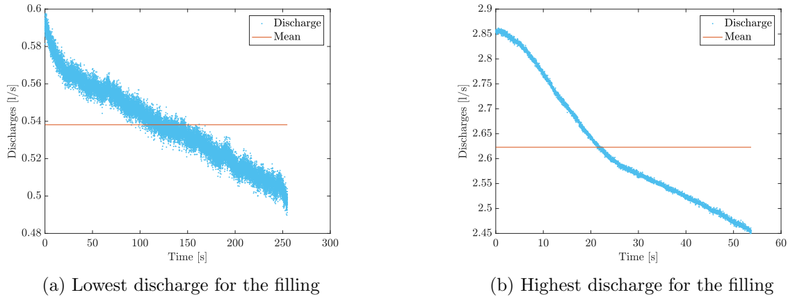
FIG. 22 Discharges of configuration one and four for the filling
