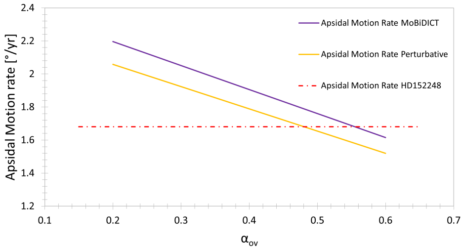
Figure 4.6: Evolution of the apsidal motion rate with respect to \alpha_{ov} .
