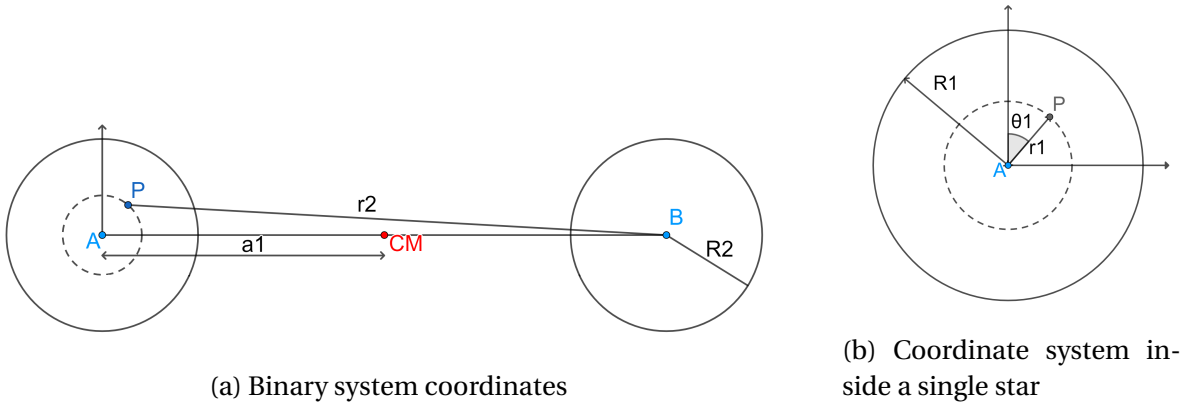
Figure 2.3: Illustration of the coordinate system used for the theoretical developments. A is the primary star, and B is the companion. P is the point at which we observe some parameters. a1 is the distance between the center of mass of the system and the center of star A. R1 and R2 are the mean radius of respectively A and B. r1 and r2 are the distances from the point P respectively to the center of star A and B. \theta1 is the angle between the point P and the perpendicular axis to the line relying upon both stars' centers, passing through the center of star A.
